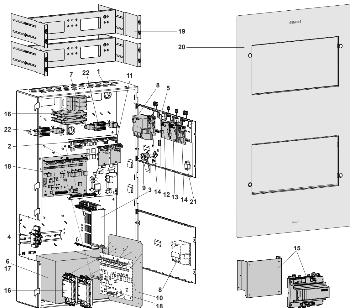
Fig. 5: FC2040 Comfort
