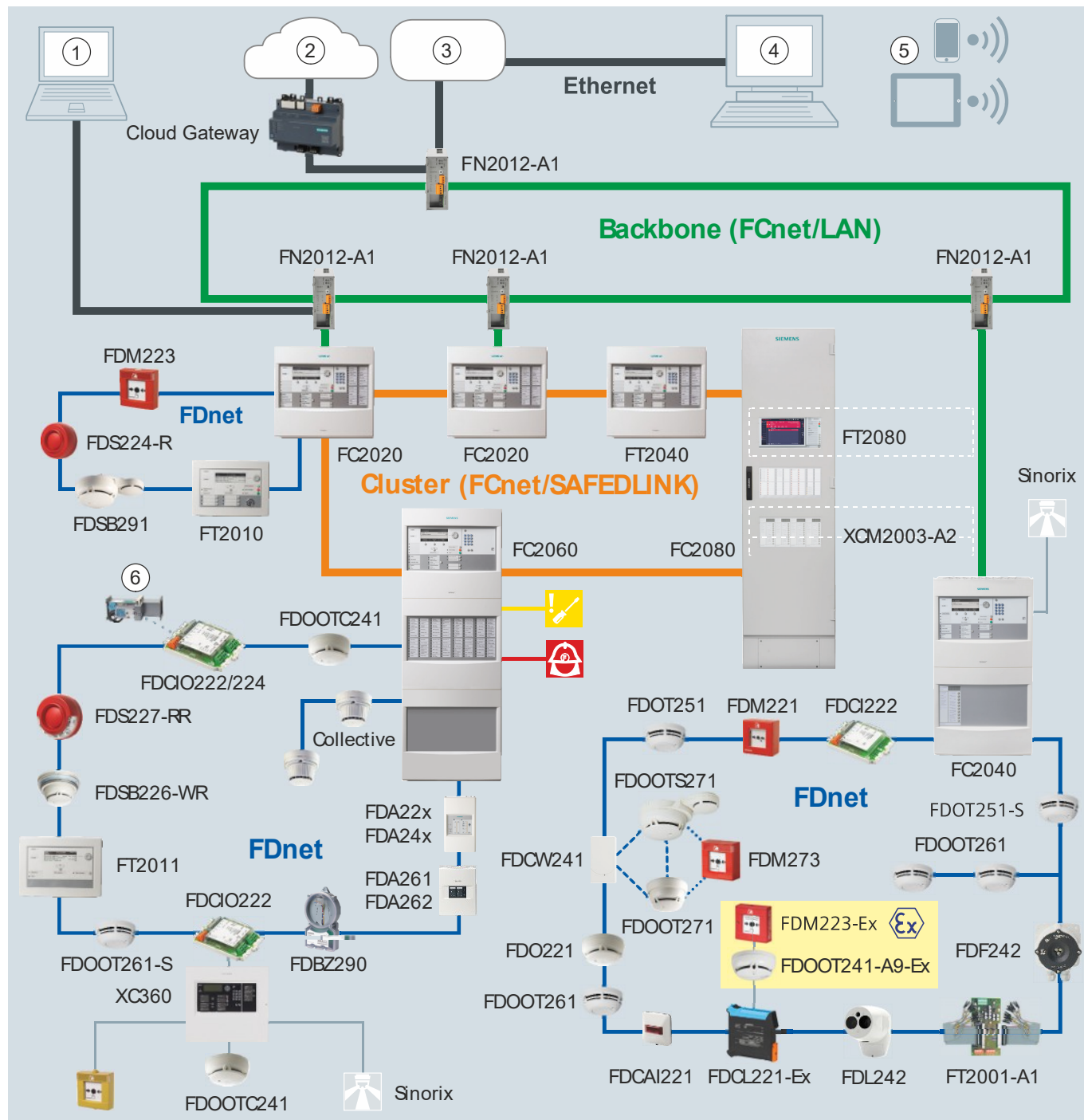
Fig. 1: System overview
