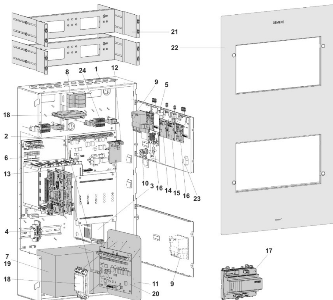
Fig. 5: Layout of FC2030
