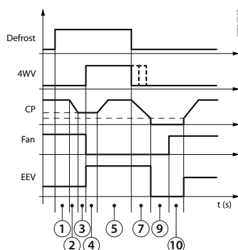
Compressor off at end defrost
