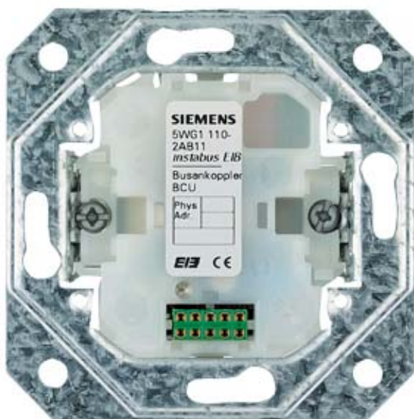
INSTABUS EIB BUS COUPLING UNIT FM 110 W. SCREW AND CLAW FIXING
